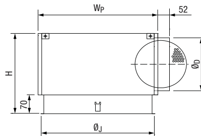
BOX-PLC/D Plenum side collar
