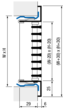
type AD300 clips and counter-frame fixing
