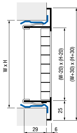
type AD780 clips and counter-frame fixing
