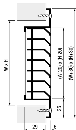
type AF350 fixing with screws
